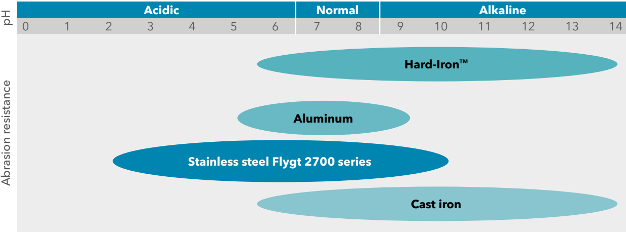
Flygt 2700 pumps can handle pH values from 2 to 10.
